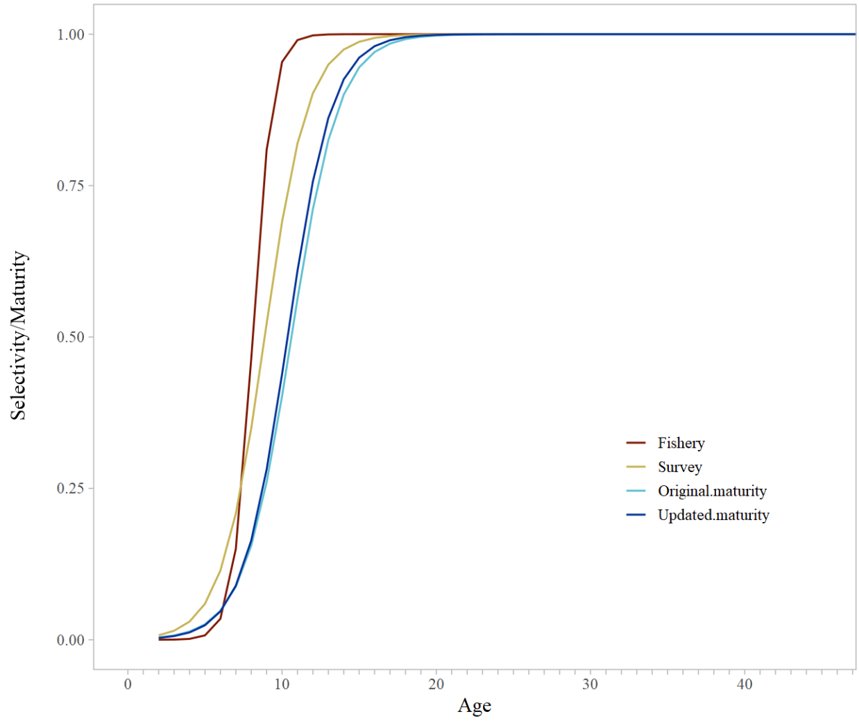
Figure 10-8. GOA northern rockfish estimated fishery and survey selectivities for the 2024 model and maturity estimates from the ADMB model and a generalized linear model with updated maturity information.
