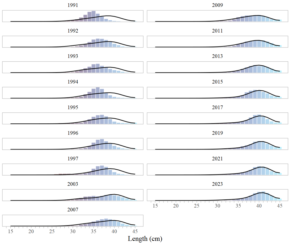
Figure 10-3. Annual fishery length composition plots. Bars are observed values, lines are estimated values.
