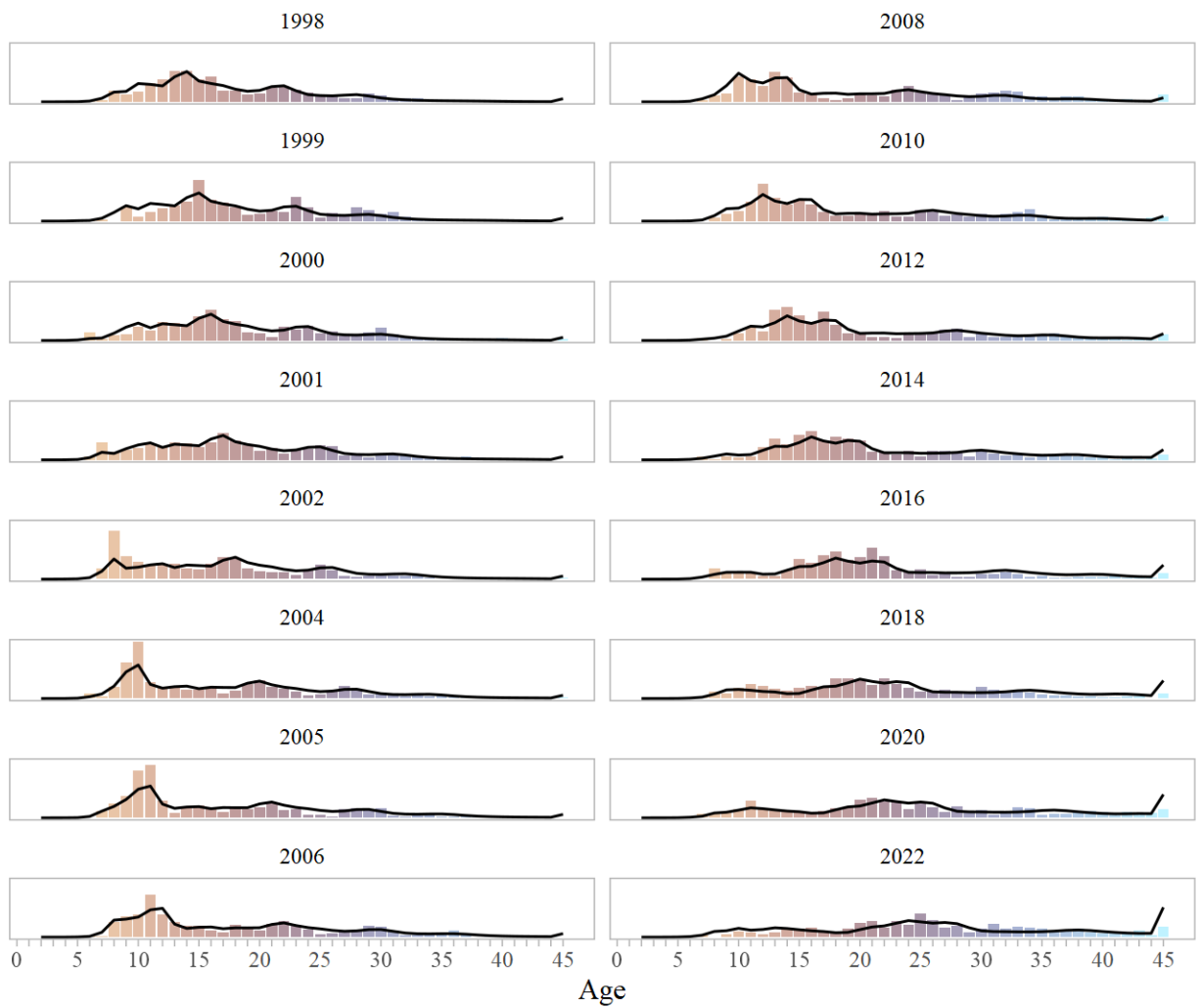
Figure 10-4. Annual fishery age composition plots. Bars are observed values, lines are estimated values.
