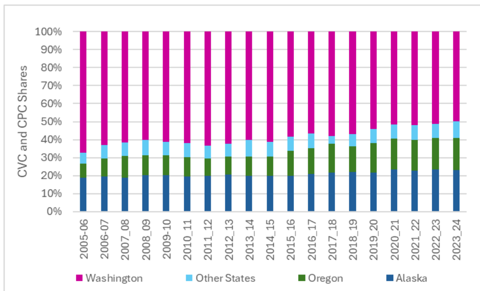
Figure 8-5 CVC and CPC QS Units Held by Year by State based on Ownership Address.
