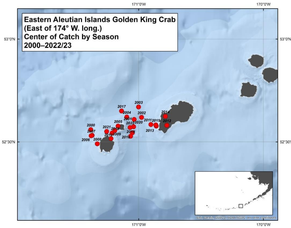
Figure 4-18 Seasonal centroid of the Eastern Aleutian Islands golden king crab fishery, 2000-2022/2023.
