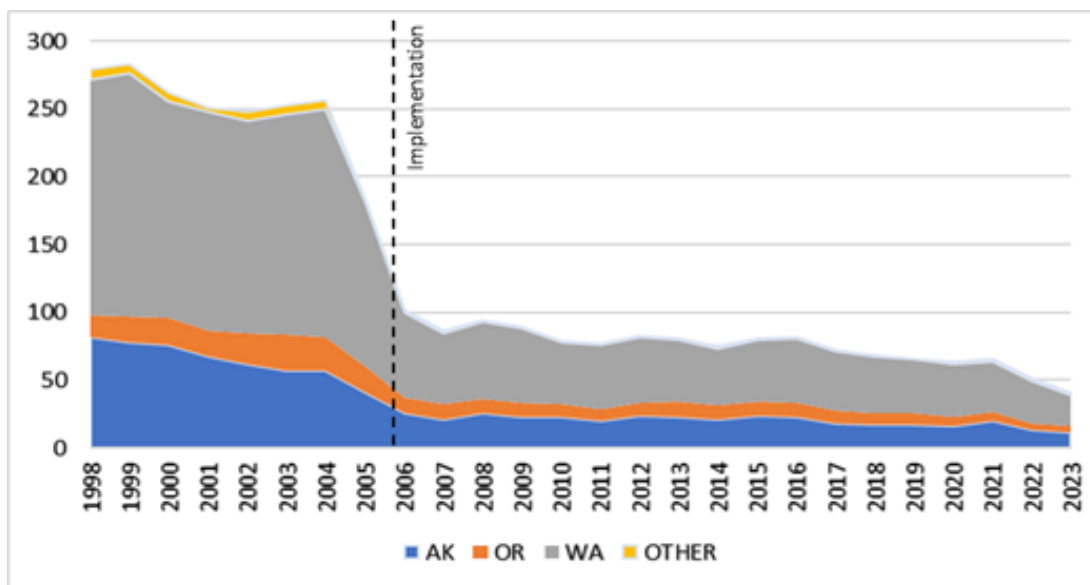
Figure 8-1 Number of Unique Catcher Vessels Engaged in the BSAI Crab Fisheries Included in the CR Program, by State, 1998-2023
